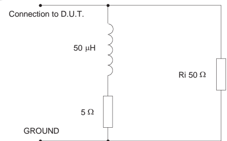
R_i = input impedance of the RFI
